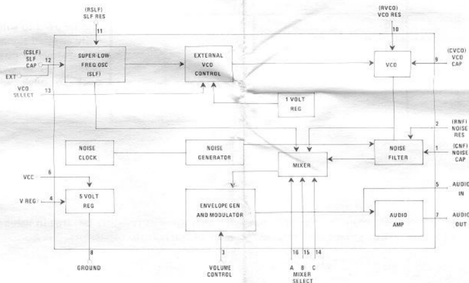
Figure 1. SN76495N BLOCK DIAGRAM
